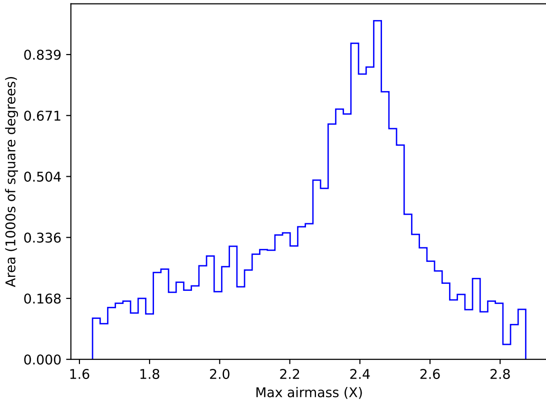
baseline_v3.3_10yrs WFD r band: Max airmass
