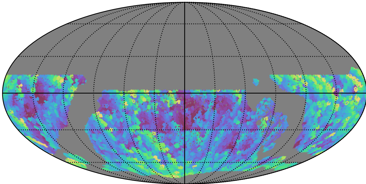
baseline_v3.3_10yrs WFD g band: Max airmass
