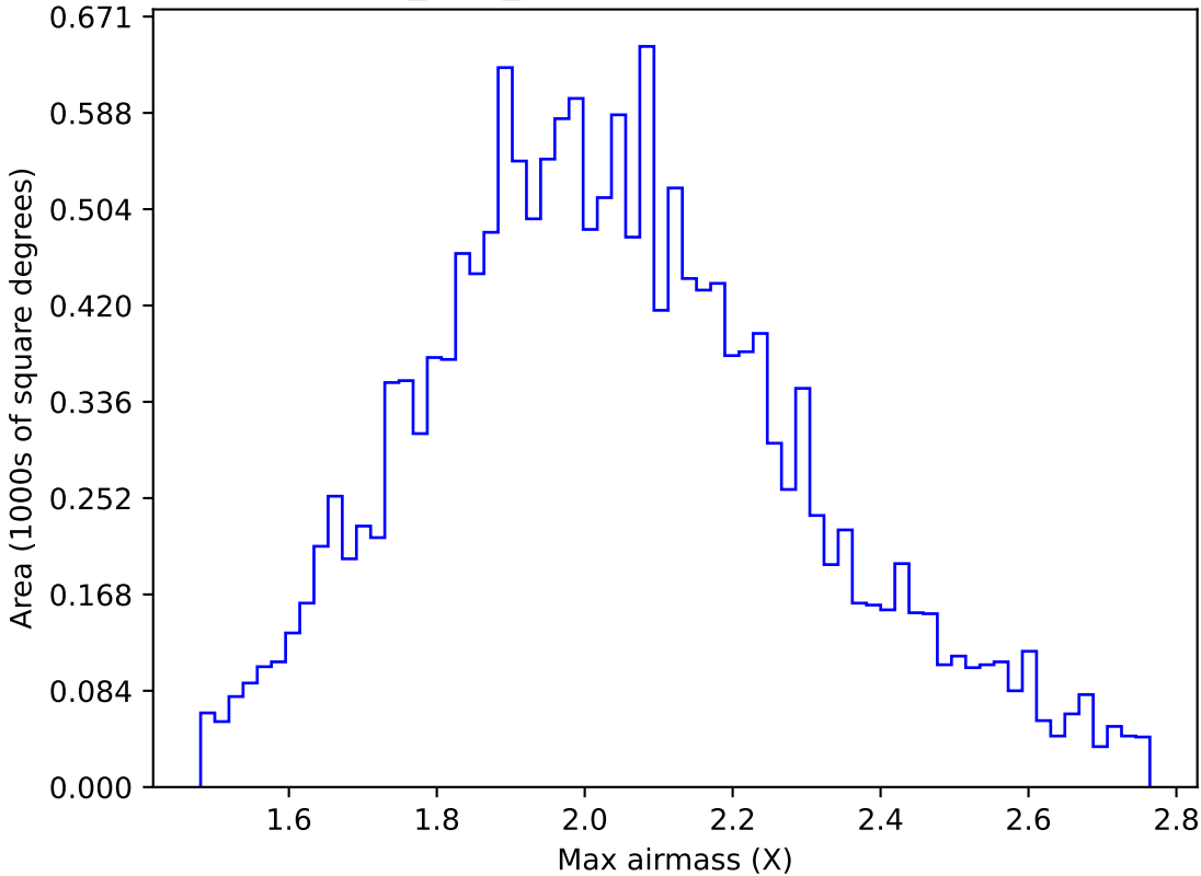
baseline_v3.3_10yrs WFD g band: Max airmass
