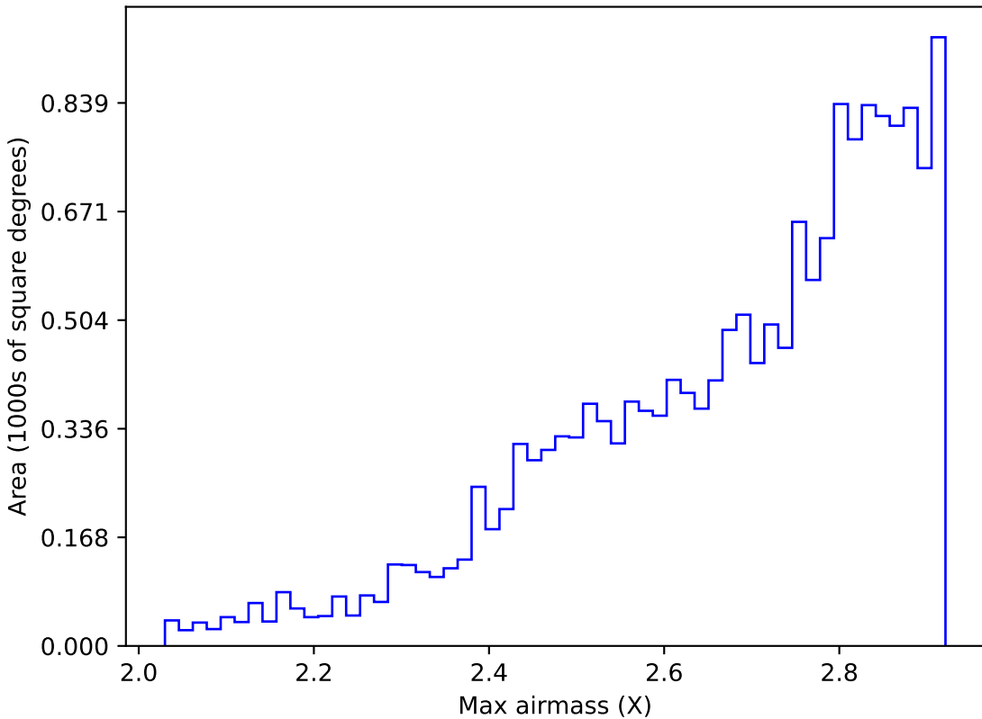
baseline_v3.3_10yrs WFD all bands: Max airmass
