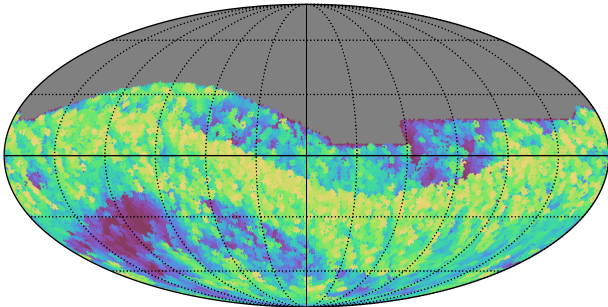
baseline_v3.3_10yrs All sky z band: Max airmass
