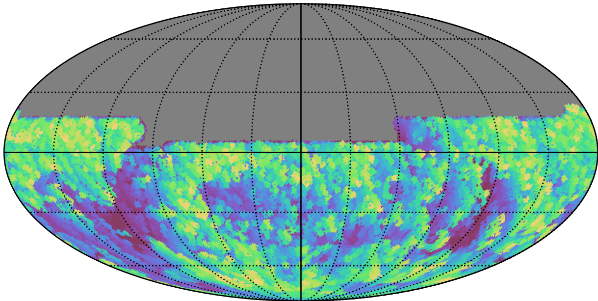
baseline_v3.3_10yrs All sky y band: Max airmass
