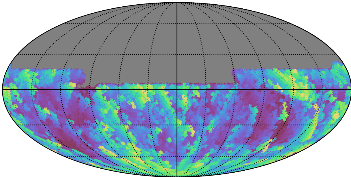
baseline_v3.3_10yrs All sky u band: Max airmass
