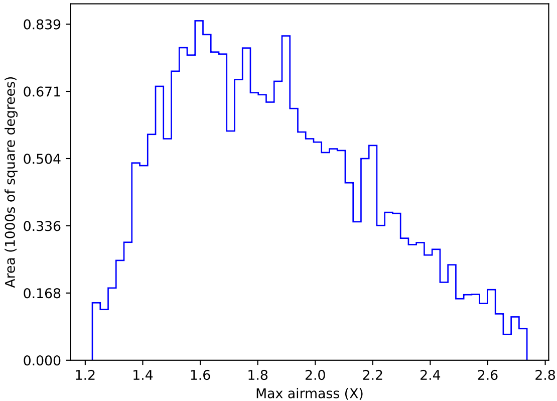
baseline_v3.3_10yrs All sky u band: Max airmass
