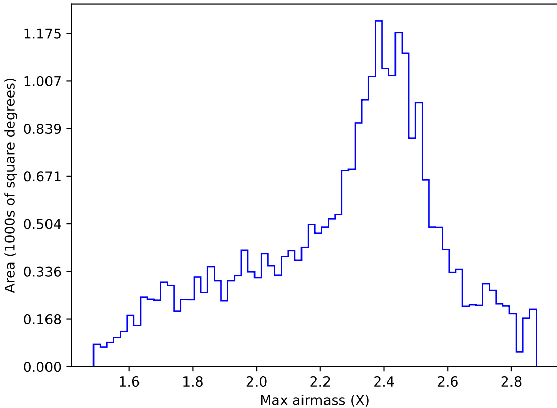
baseline_v3.3_10yrs All sky r band: Max airmass
