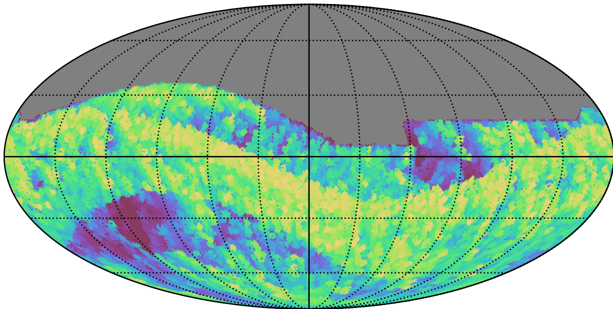
baseline_v3.3_10yrs All sky i band: Max airmass
