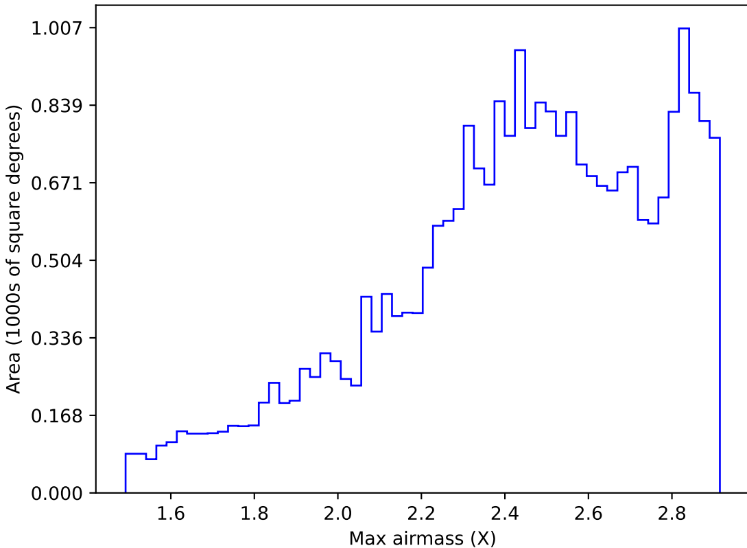
baseline_v3.3_10yrs All sky i band: Max airmass
