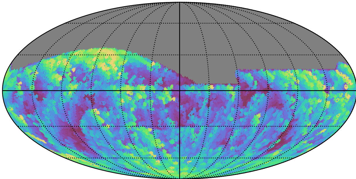
baseline_v3.3_10yrs All sky g band: Max airmass
