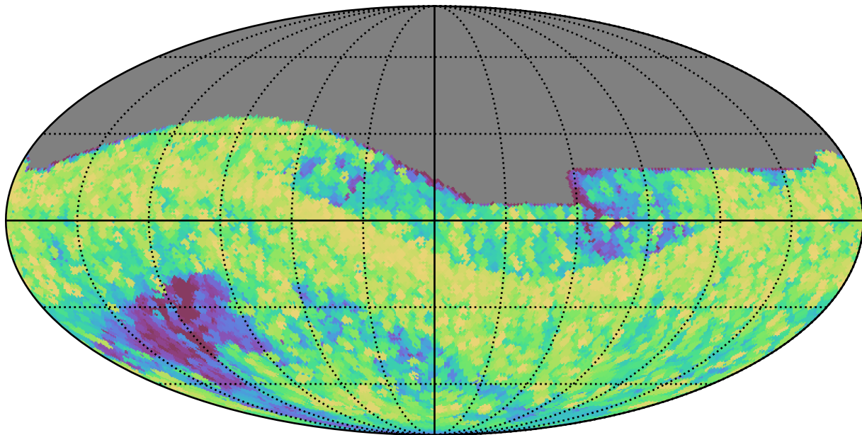
baseline_v3.3_10yrs All sky all bands: Max airmass
