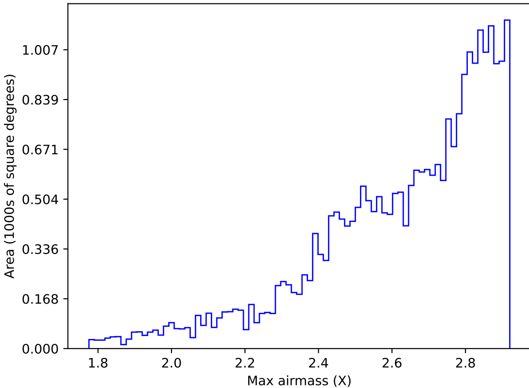
baseline_v3.3_10yrs All sky all bands: Max airmass
