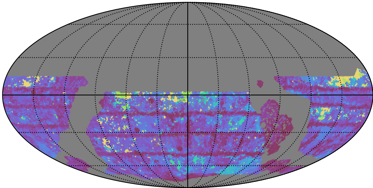
baseline_v3.3_10yrs WFD z band: Max Inter-Night Gap
