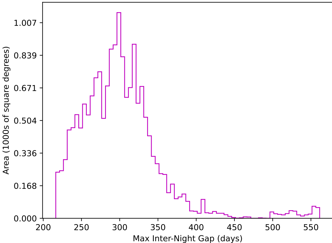
baseline_v3.3_10yrs WFD z band: Max Inter-Night Gap
