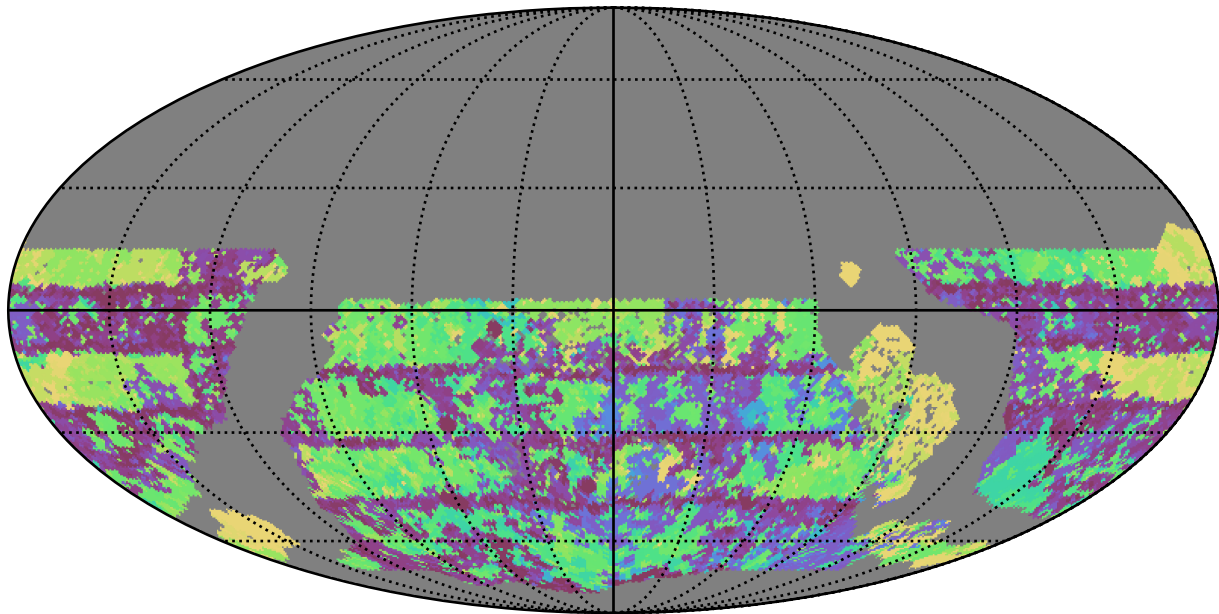
baseline_v3.3_10yrs WFD u band: Max Inter-Night Gap
