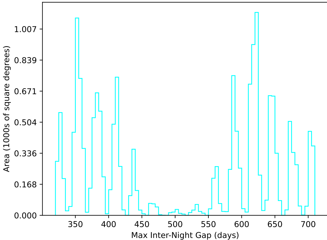
baseline_v3.3_10yrs WFD u band: Max Inter-Night Gap
