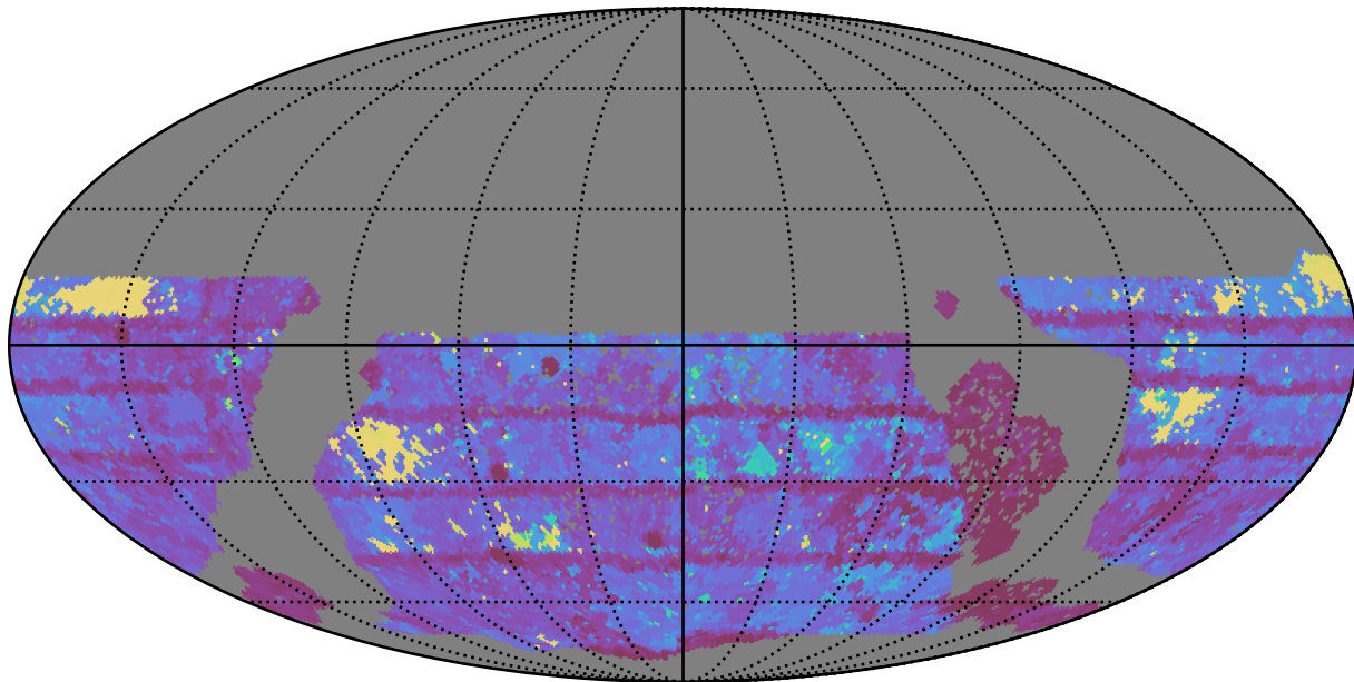
baseline_v3.3_10yrs WFD r band: Max Inter-Night Gap
