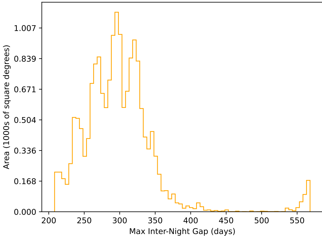
baseline_v3.3_10yrs WFD r band: Max Inter-Night Gap
