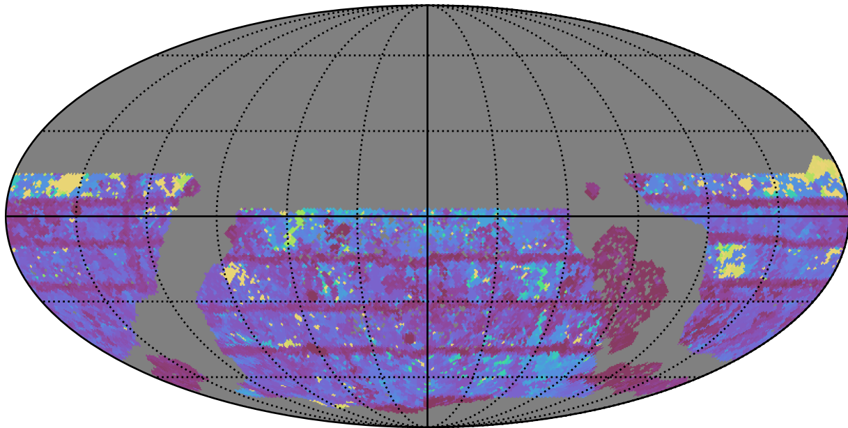
baseline_v3.3_10yrs WFD i band: Max Inter-Night Gap
