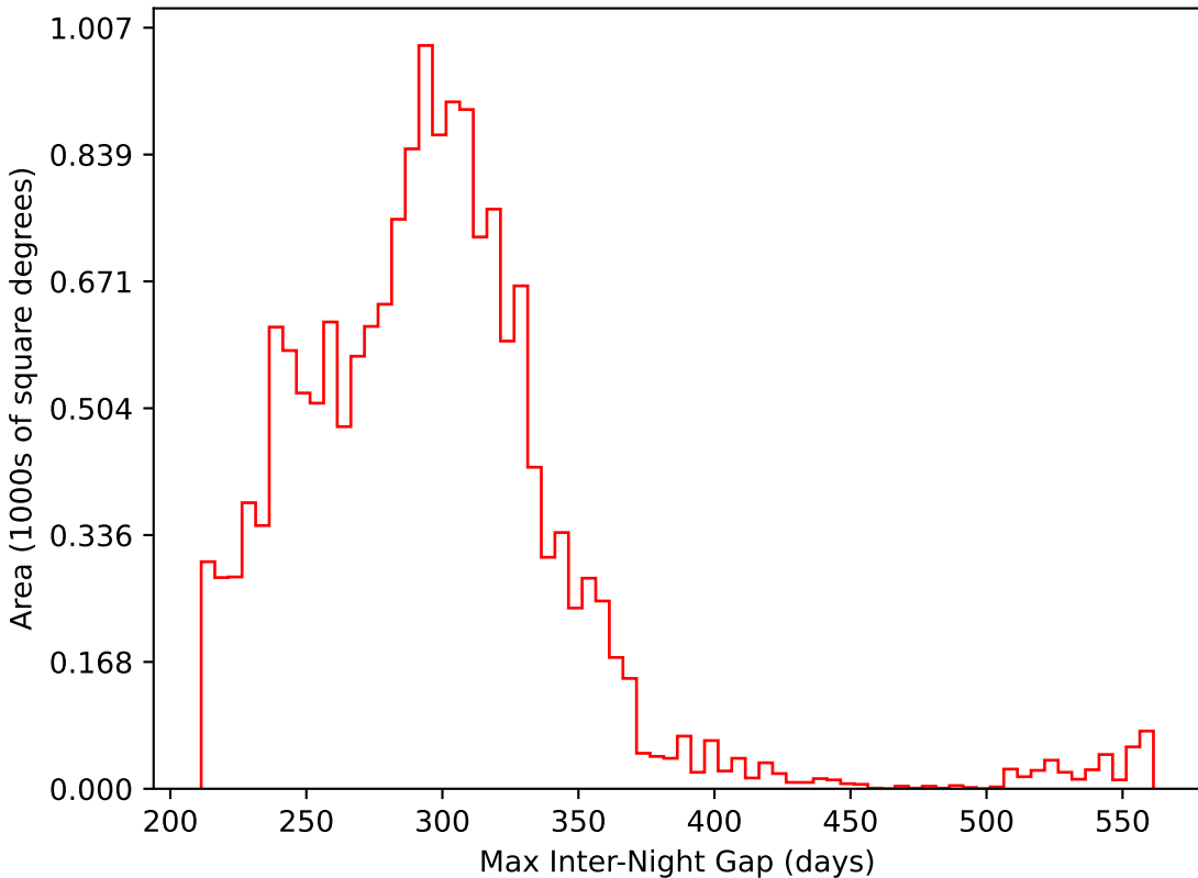
baseline_v3.3_10yrs WFD i band: Max Inter-Night Gap
