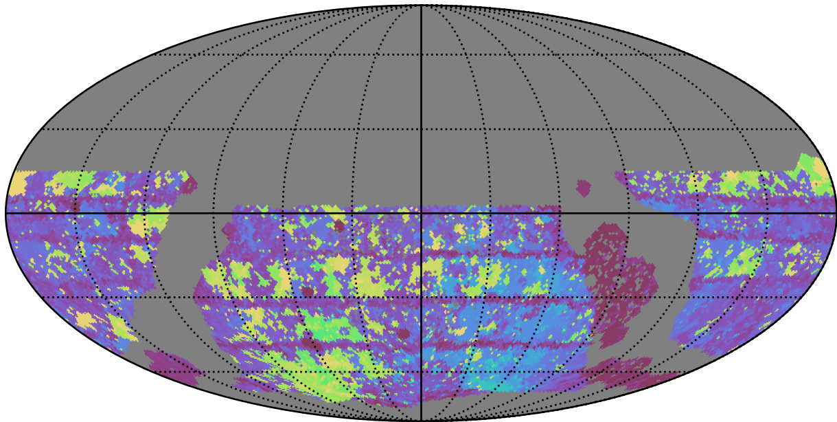
baseline_v3.3_10yrs WFD g band: Max Inter-Night Gap
