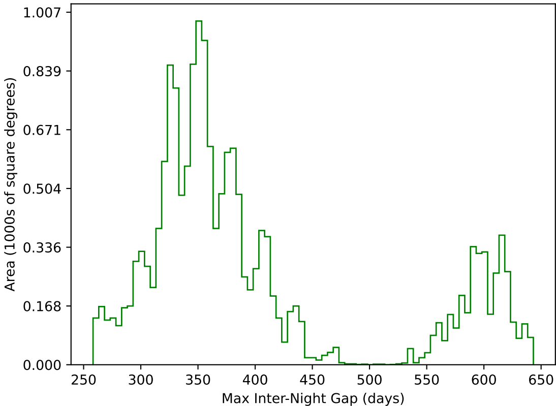
baseline_v3.3_10yrs WFD g band: Max Inter-Night Gap
