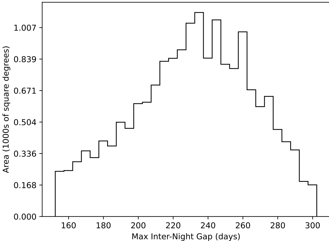
baseline_v3.3_10yrs WFD all bands: Max Inter-Night Gap
