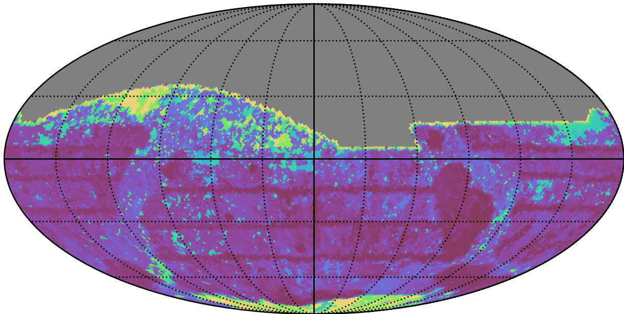
baseline_v3.3_10yrs All sky z band: Max Inter-Night Gap
