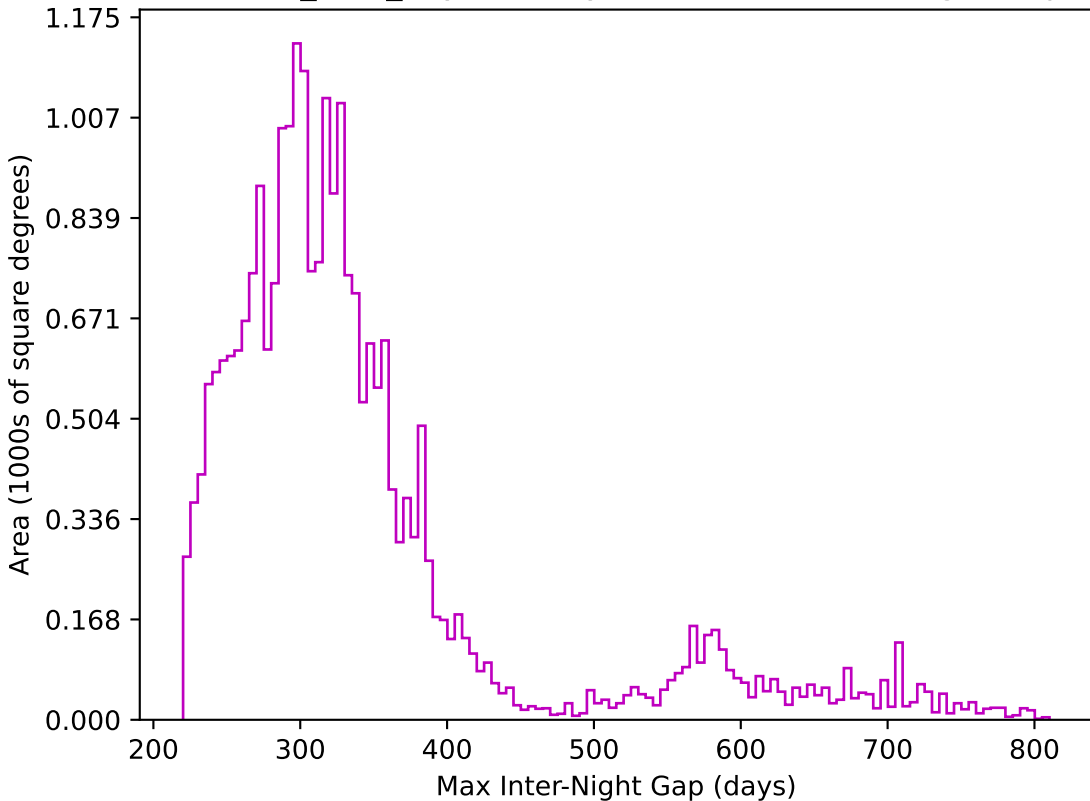
baseline_v3.3_10yrs All sky z band: Max Inter-Night Gap
