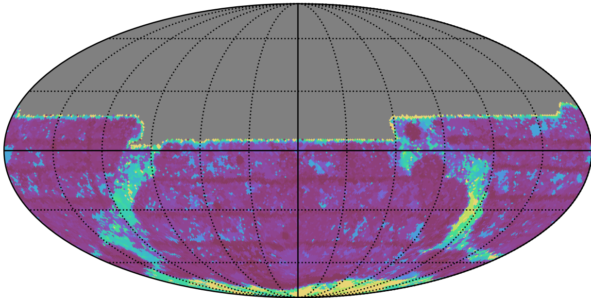
baseline_v3.3_10yrs All sky y band: Max Inter-Night Gap
