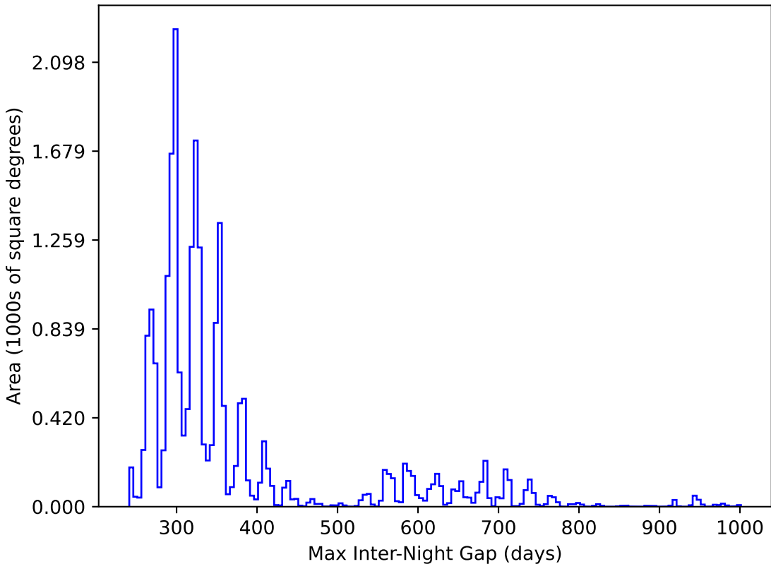
baseline_v3.3_10yrs All sky y band: Max Inter-Night Gap
