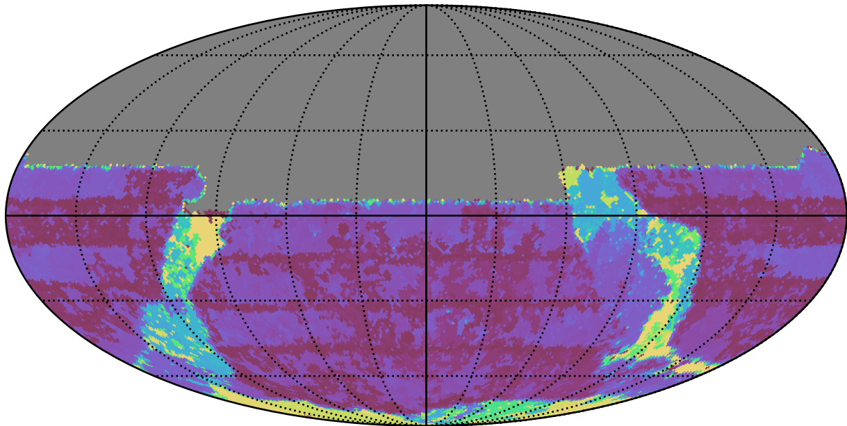
baseline_v3.3_10yrs All sky u band: Max Inter-Night Gap
