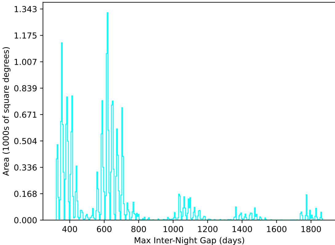
baseline_v3.3_10yrs All sky u band: Max Inter-Night Gap
