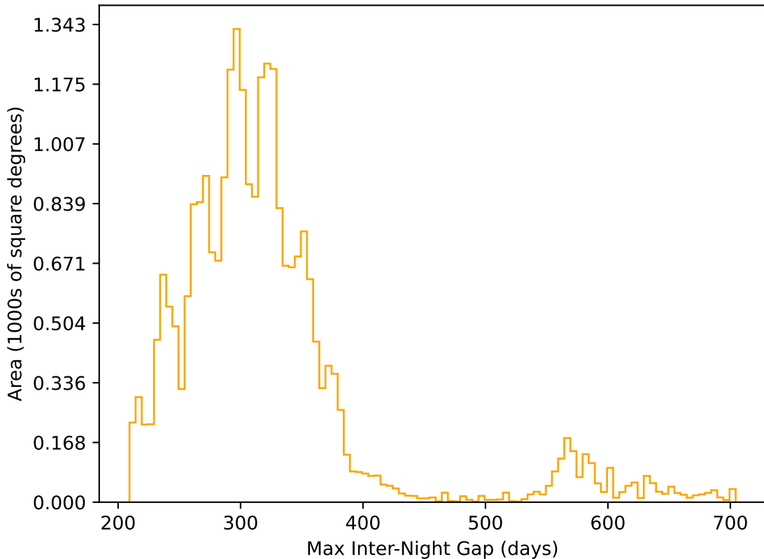
baseline_v3.3_10yrs All sky r band: Max Inter-Night Gap
