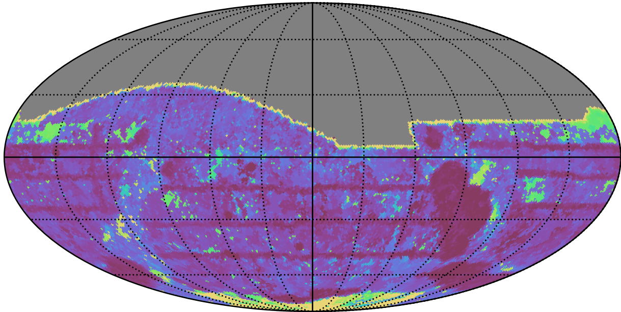
baseline_v3.3_10yrs All sky i band: Max Inter-Night Gap
