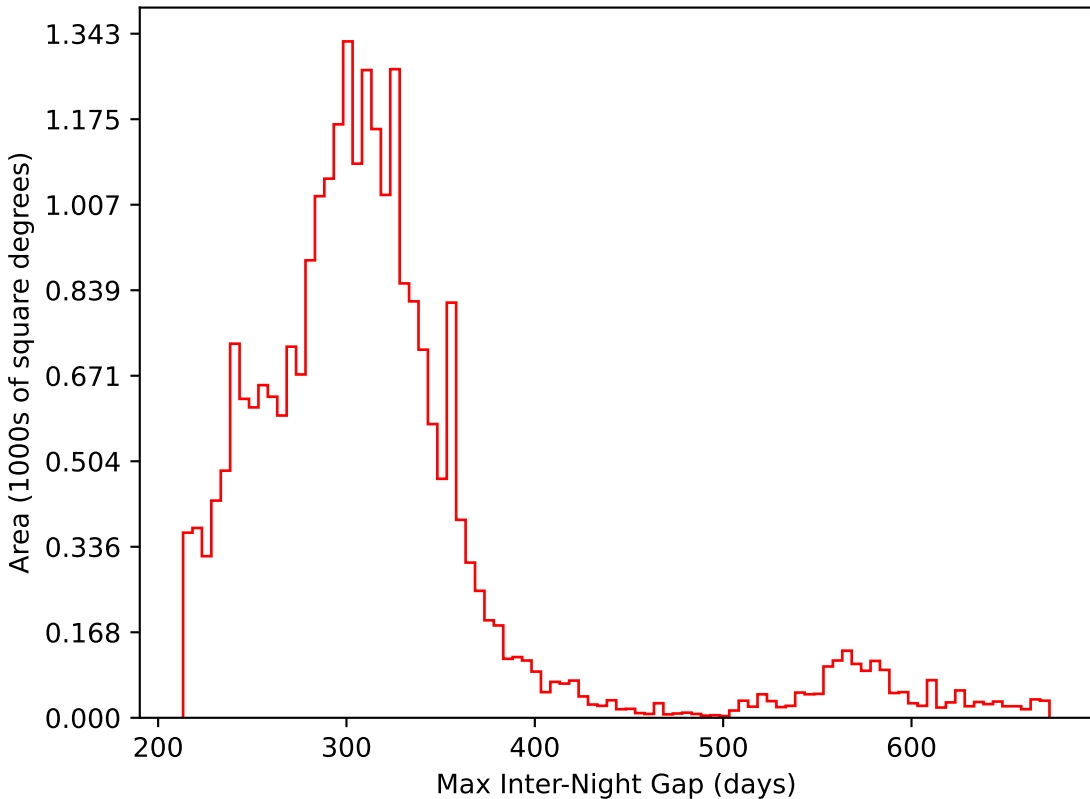
baseline_v3.3_10yrs All sky i band: Max Inter-Night Gap
