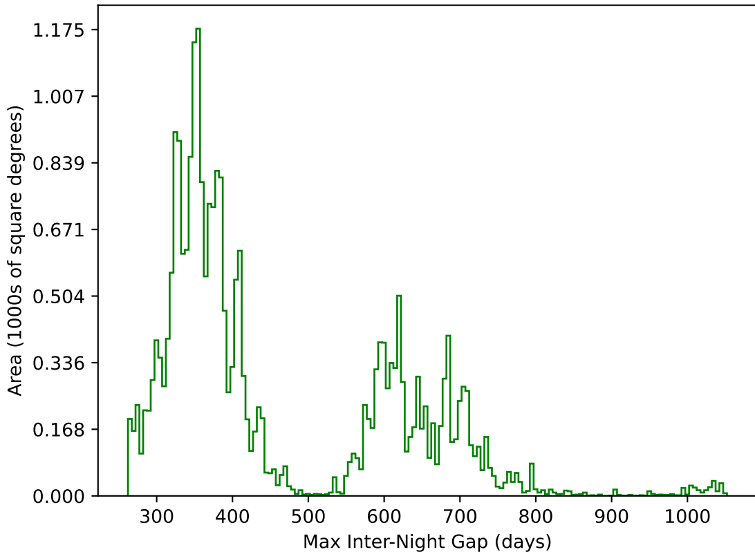
baseline_v3.3_10yrs All sky g band: Max Inter-Night Gap
