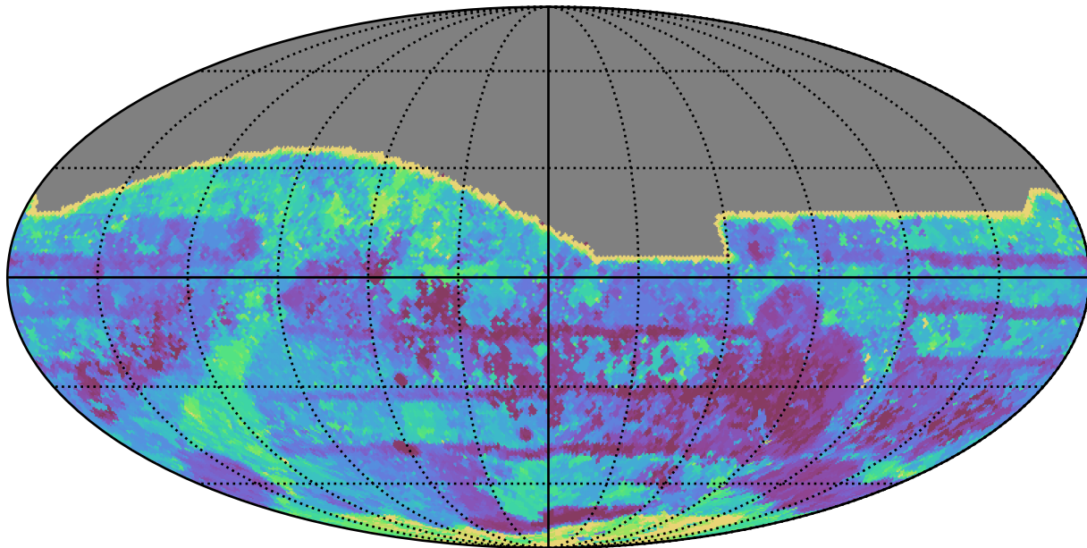
baseline_v3.3_10yrs All sky all bands: Max Inter-Night Gap
