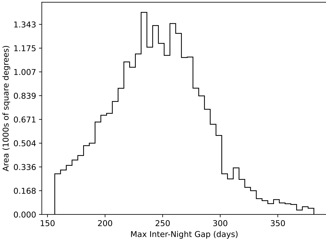
baseline_v3.3_10yrs All sky all bands: Max Inter-Night Gap
