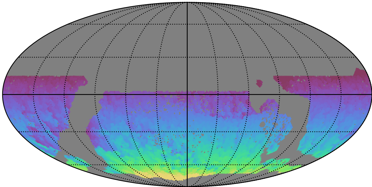
baseline_v3.3_10yrs WFD all bands: Max HA
