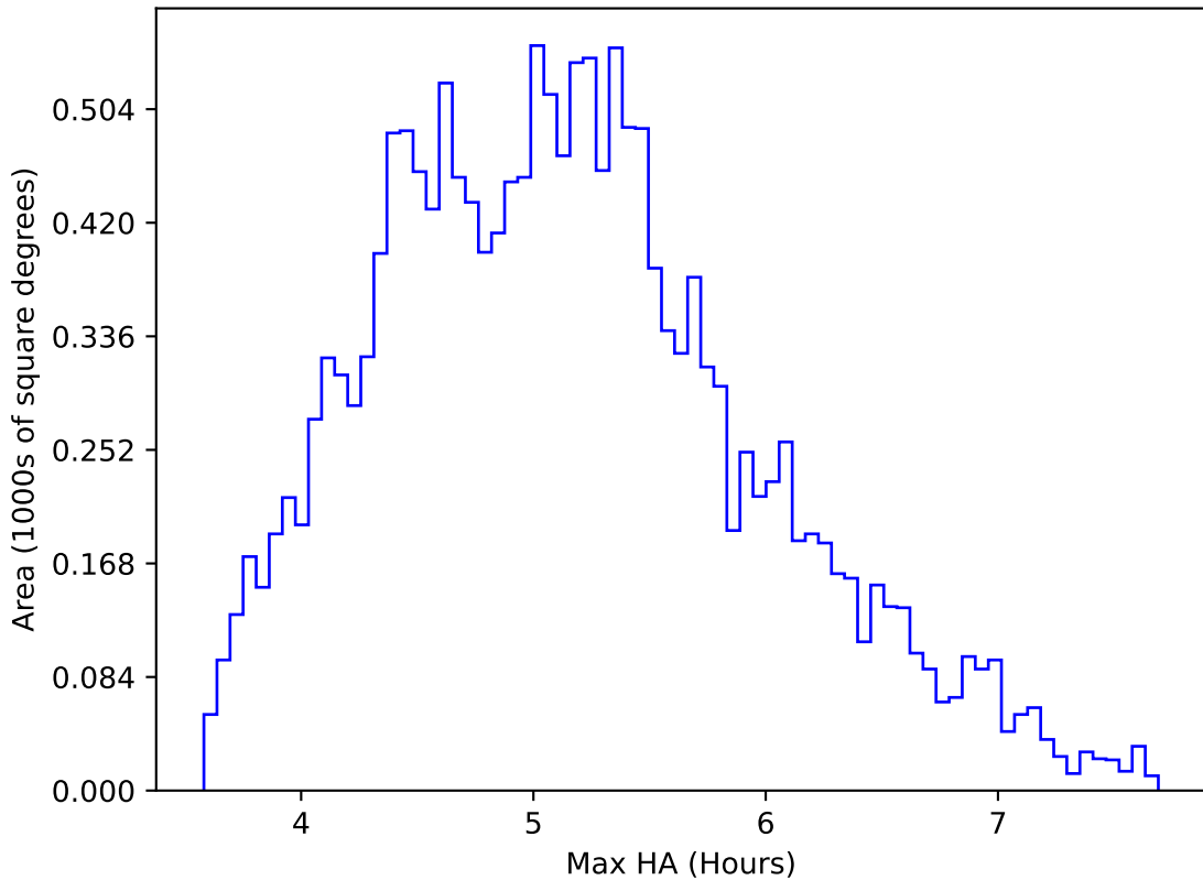
baseline_v3.3_10yrs WFD all bands: Max HA
