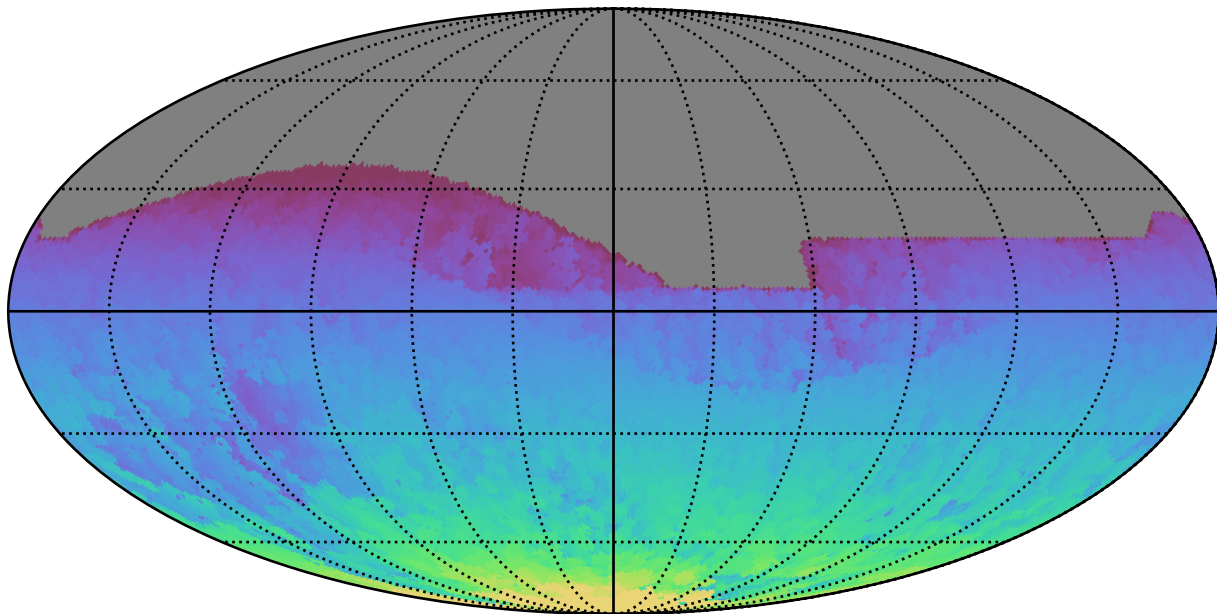
baseline_v3.3_10yrs All sky all bands: Max HA
