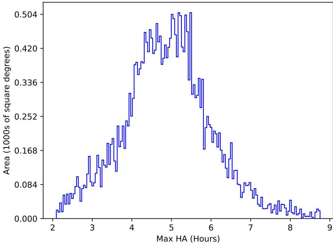
baseline_v3.3_10yrs All sky all bands: Max HA
