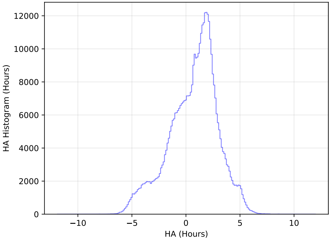
baseline_v3.3_10yrs WFD z band: HA Histogram
