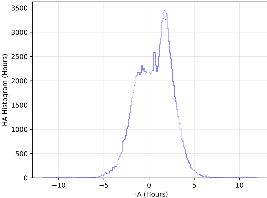
baseline_v3.3_10yrs WFD u band: HA Histogram
