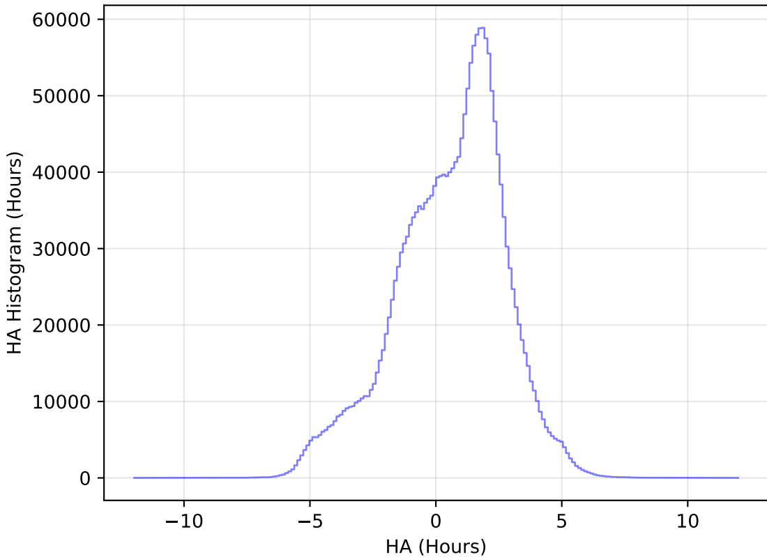
baseline_v3.3_10yrs All sky all bands: HA Histogram
