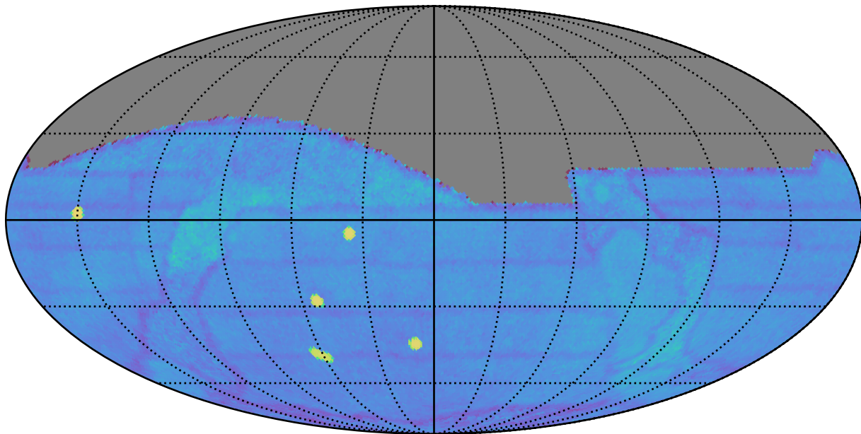
baseline_v3.3_10yrs gri All sky: Fraction of visits with a revisit < 60 min
