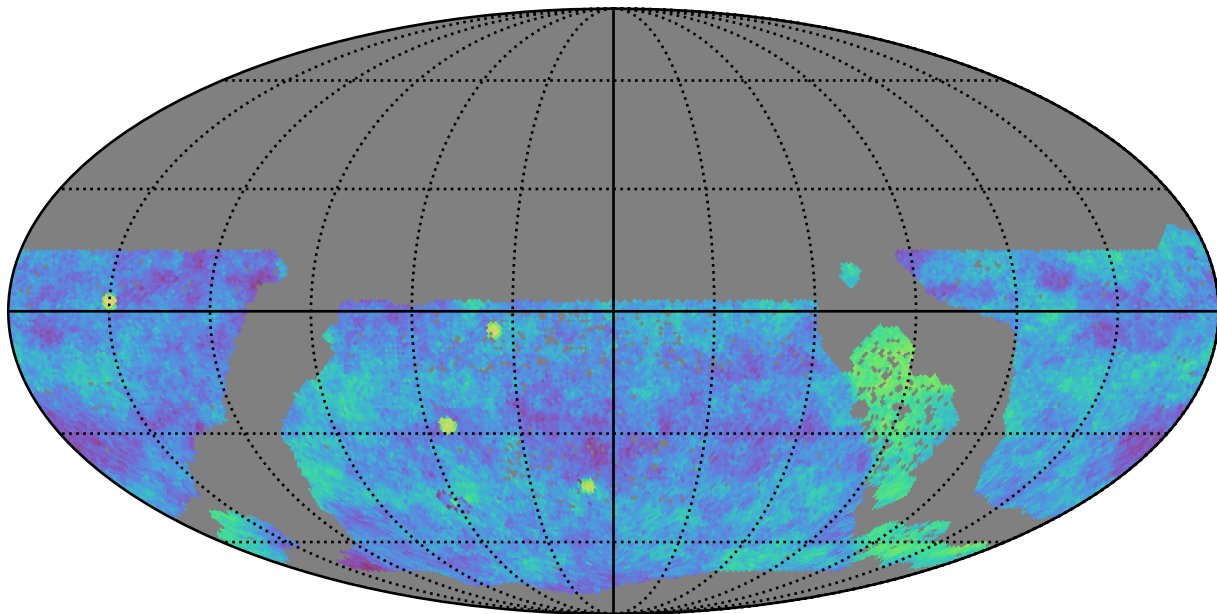
baseline_v3.3_10yrs gri WFD: Fraction of visits in pairs (20-90 min)
