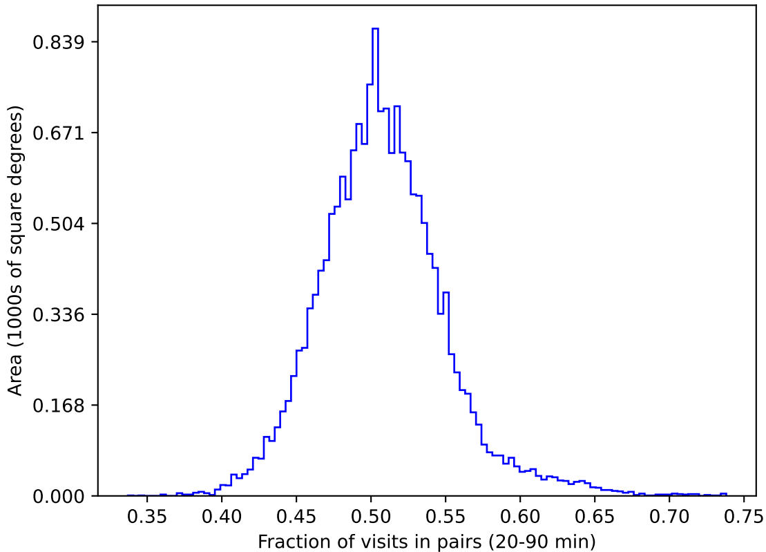
baseline_v3.3_10yrs gri WFD: Fraction of visits in pairs (20-90 min)
