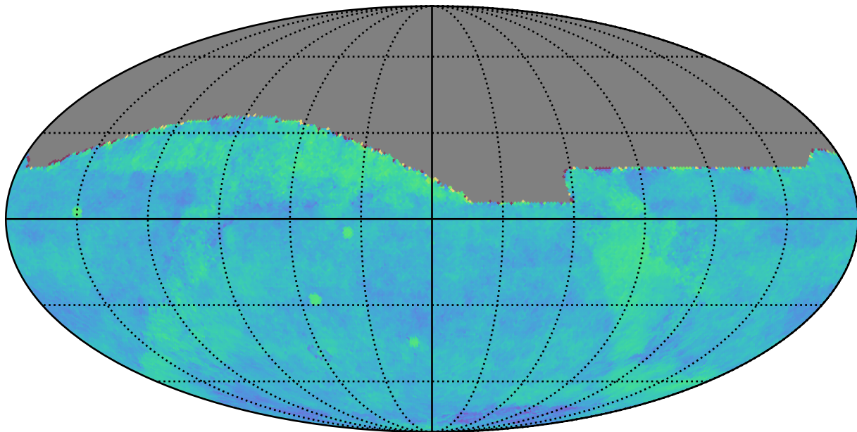
baseline_v3.3_10yrs gri All sky: Fraction of visits in pairs (20-90 min)
