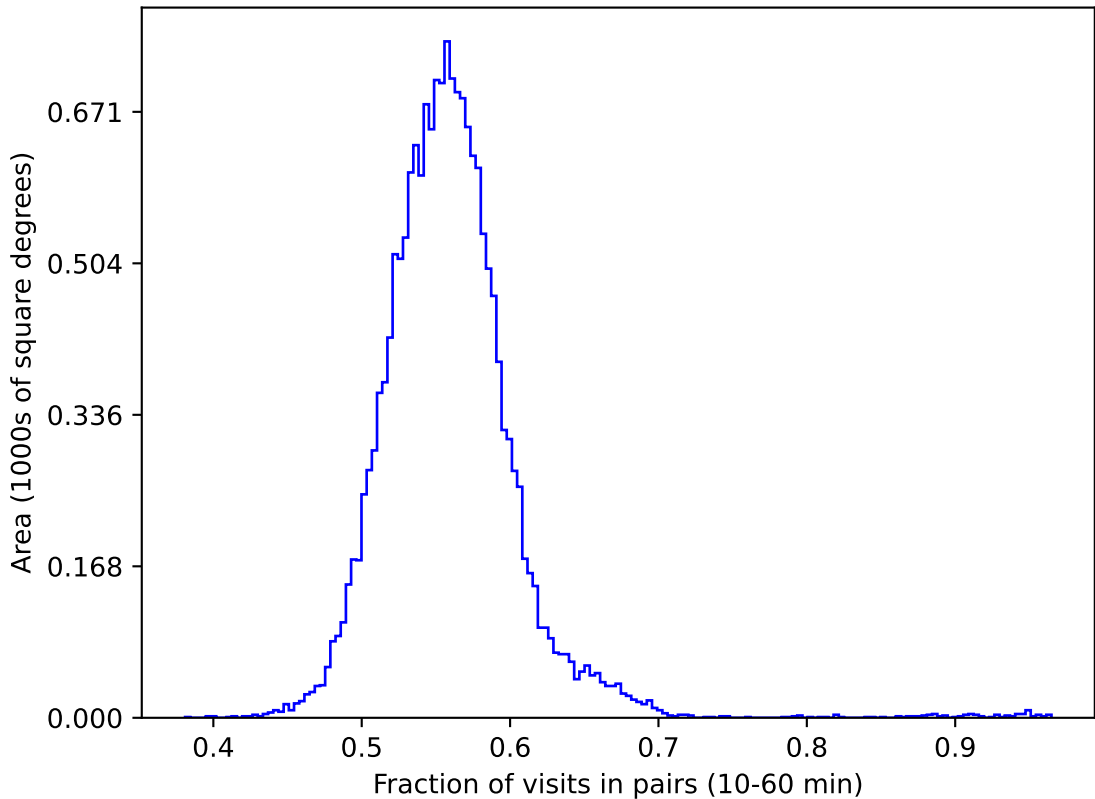
baseline_v3.3_10yrs gri WFD: Fraction of visits in pairs (10-60 min)
