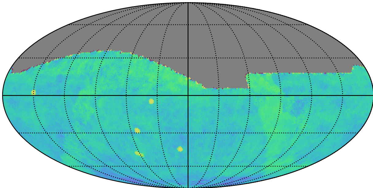
baseline_v3.3_10yrs gri All sky: Fraction of visits in pairs (10-60 min)
